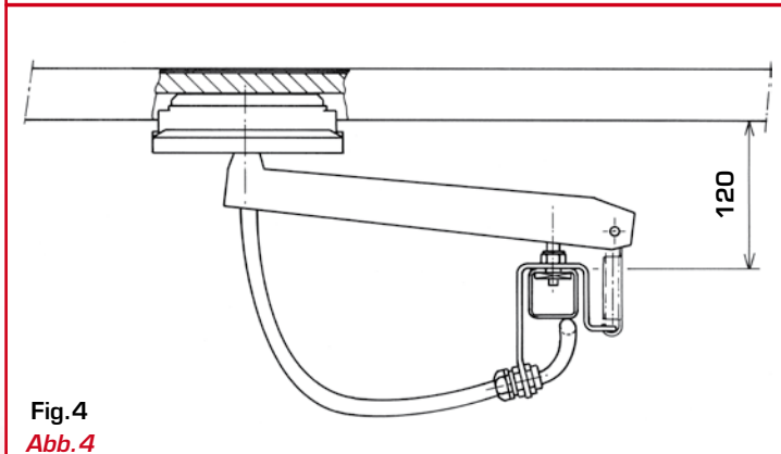
Fig. 4 Current collector: LMC 150.C1
