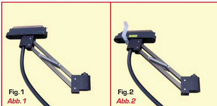
Fig. 1 CURRENT COLLECTOR: CMC150.C1
